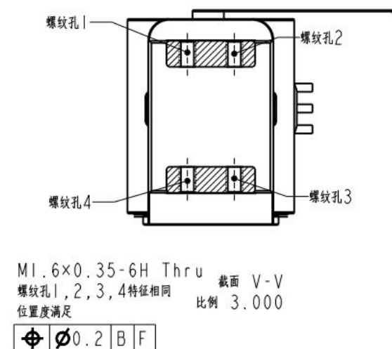
L-Bracket Mounting Hole Detail
